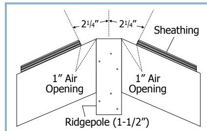
Ridgepole Diagram
