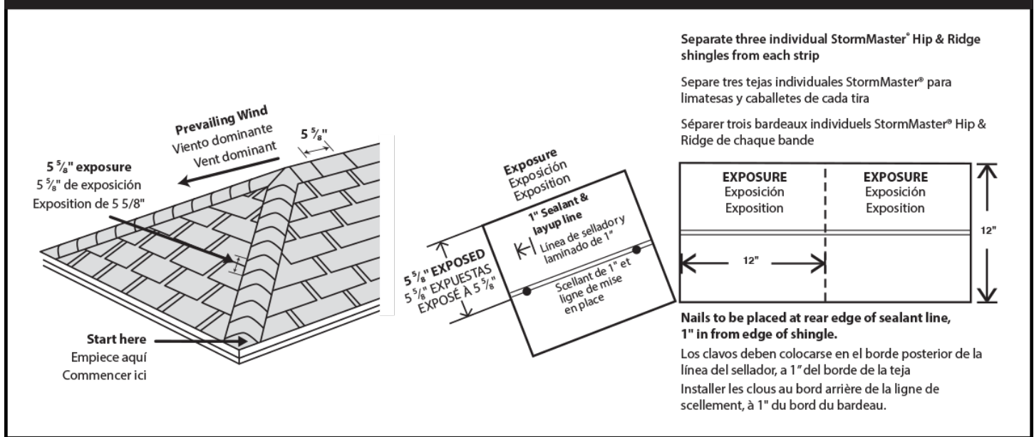
DIAGRAM 6 HIP & RIDGE
